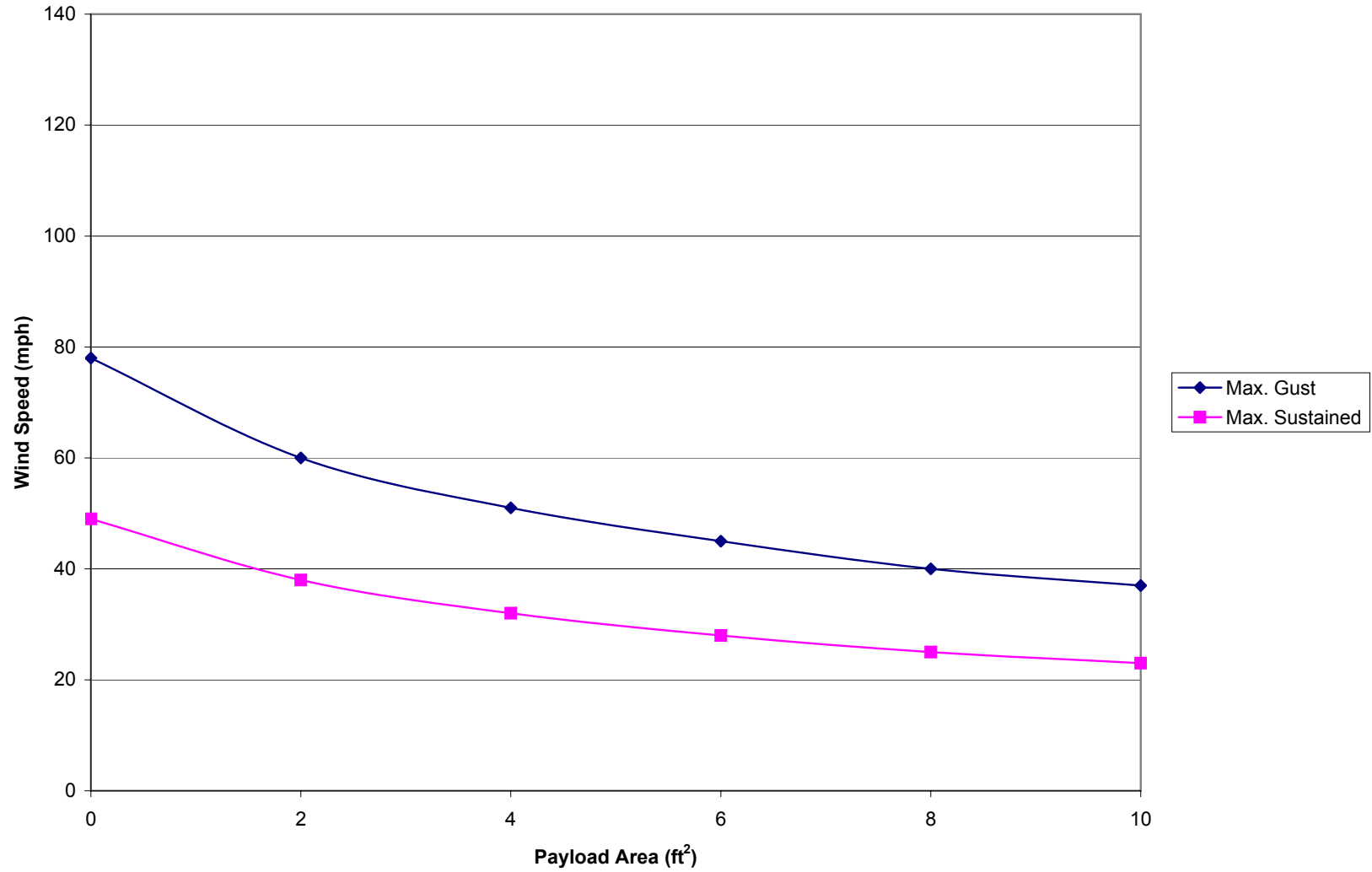
Wind Speed vs Payload Area 8-30 Non-locking Mast
