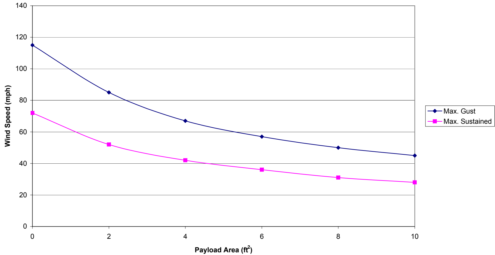
Wind Speed vs. Payload Area 5-20 Non-locking Mast
